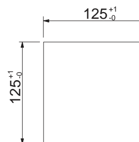
Cut-Out Dimensions
